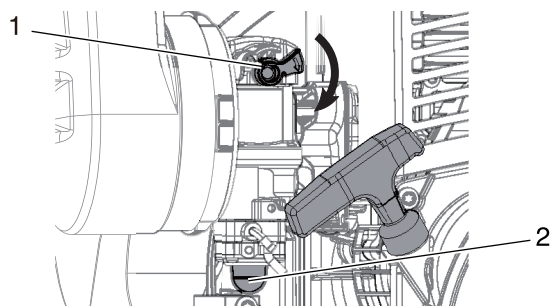
1. Choke lever
