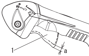
1. Throttle trigger
