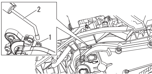
1. Grease fitting
