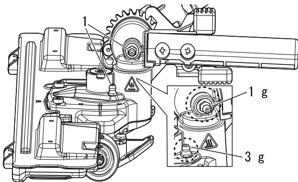
1. Grease fitting
