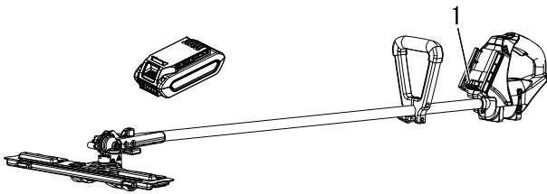
1. Battery compartment
