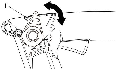
1. Cruise control lever 3. Slow speed 2. Blower stop 4. Fast speed
