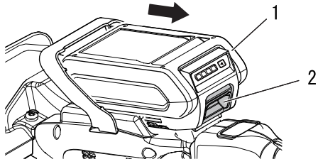
1. Battery
