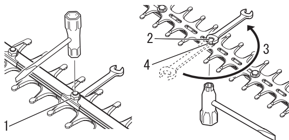
1. Locknut 2. Bolt
