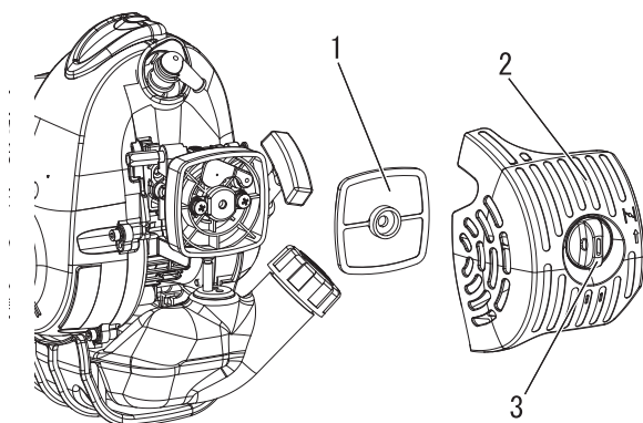
1. Air filter
