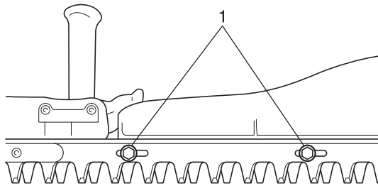
1. Bolt slots
