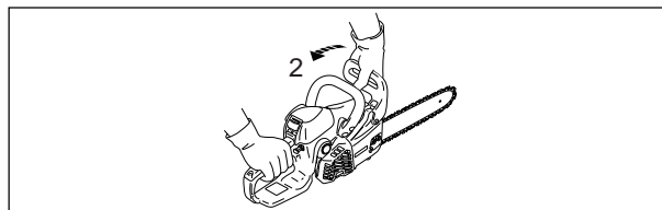
2. Release chain brake
